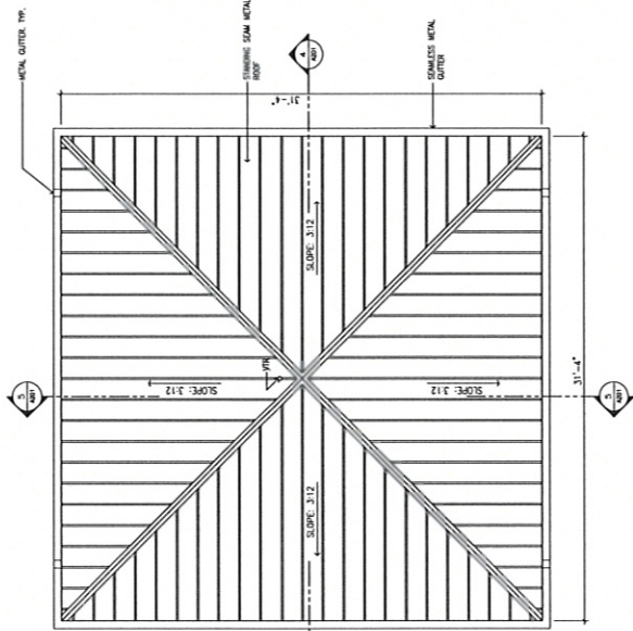
2 ROOF PLAN A101 SCALE: 1/4" = 1'-0"
