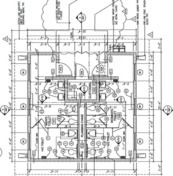
1 FLOOR PLAN A101 SCALE: 1/8" = 1'-0" 3/4"
